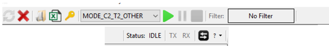
Figure 7: Main Menu
